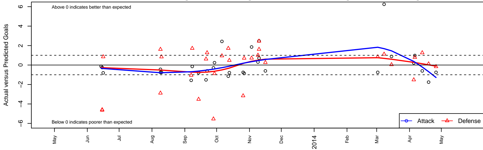
THUSC Obsidian G02 Dots are actual minus expected GF (blue circles) and GA (red triangles). Blue line is smoothed change in attack strength. Red is smoothed change in defense strength.
